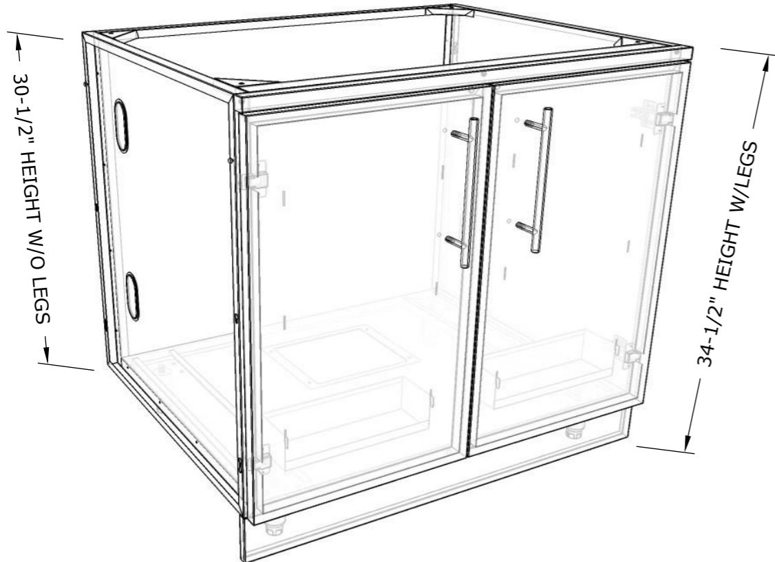
ISO VIEW
